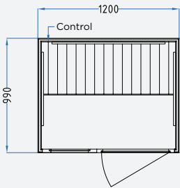
LAYOUT
